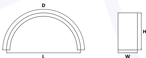
Parafanghi inox fiorettato gomma Stainless steel mudguards with texture and rubber edge
