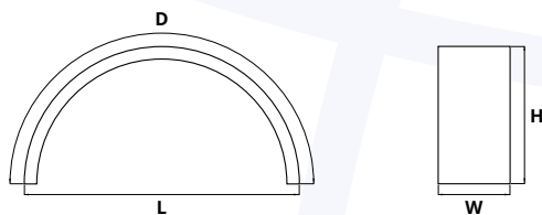
Parafanghi Interflex inox liscio gomma Stainless steel mudguards with rubber edge
